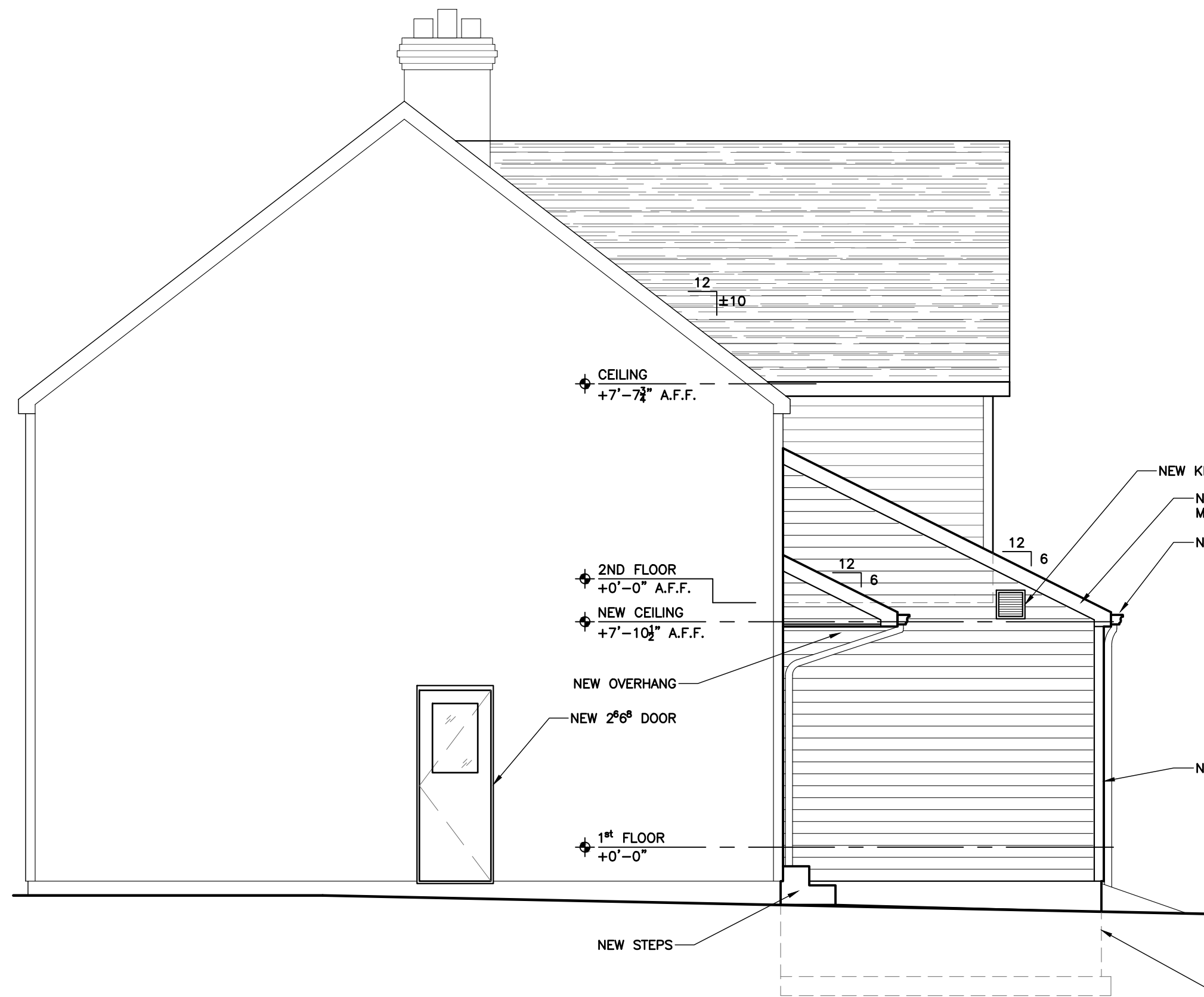
PROPOSED RIGHT ELEVATION Scale: 1/4" = 1'-0"
