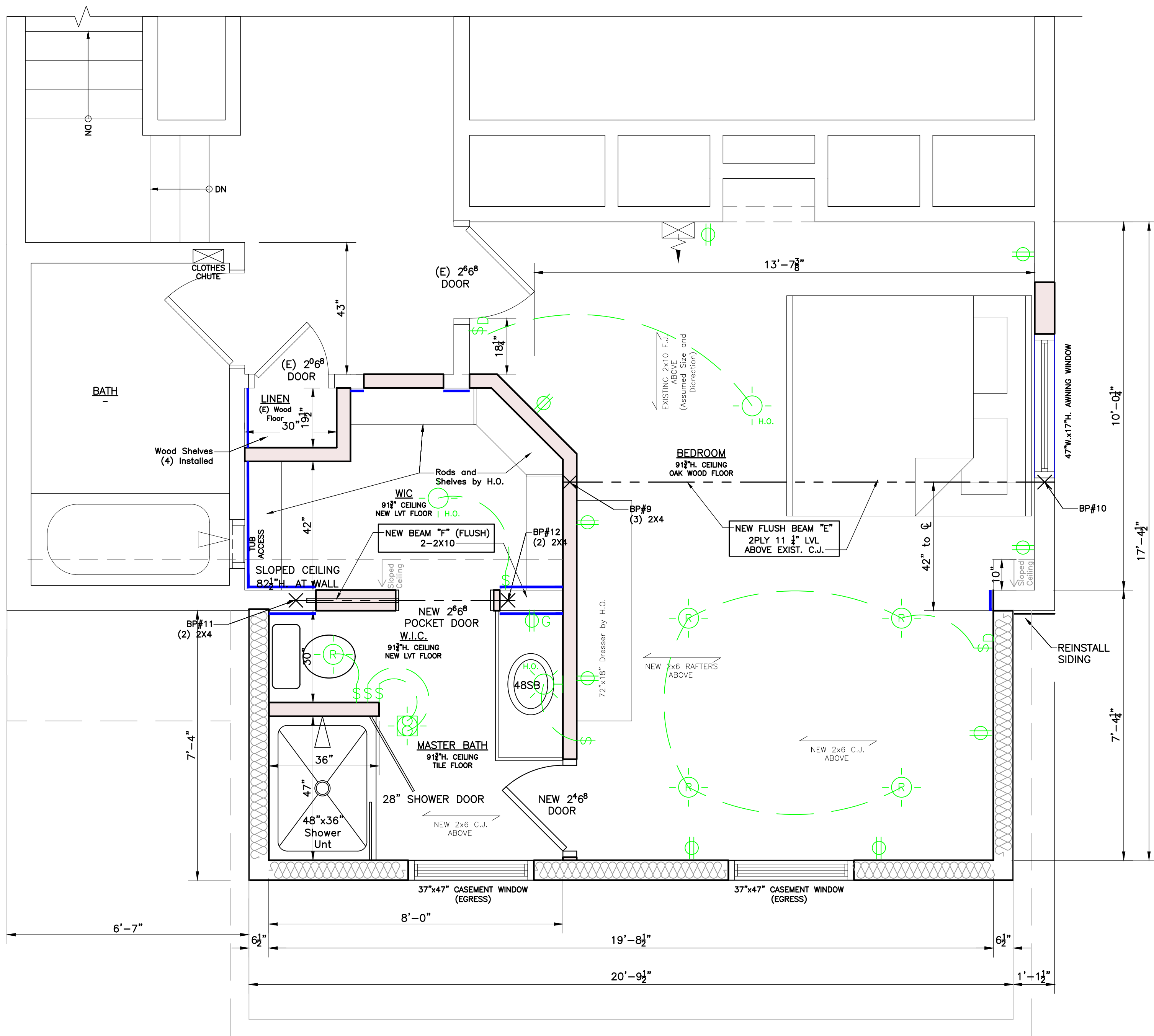
PROPOSED 2ND FLOOR PLAN Scale: 1/2" = 1'-0"
