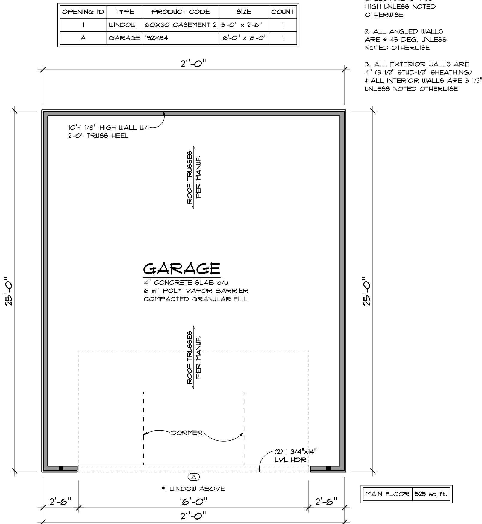
MAIN LEVEL FLOOR PLAN
