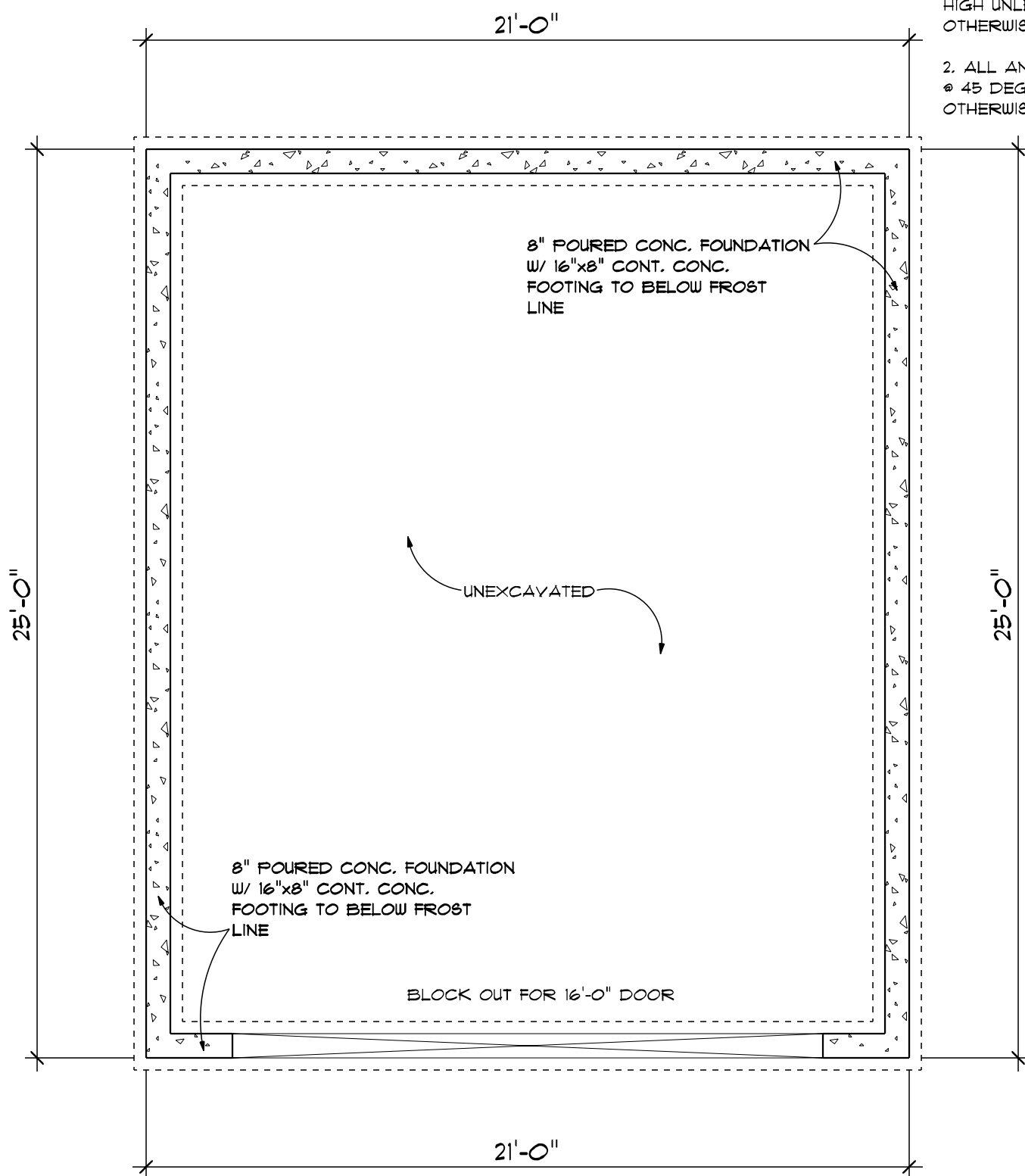
FOUNDATION PLAN
