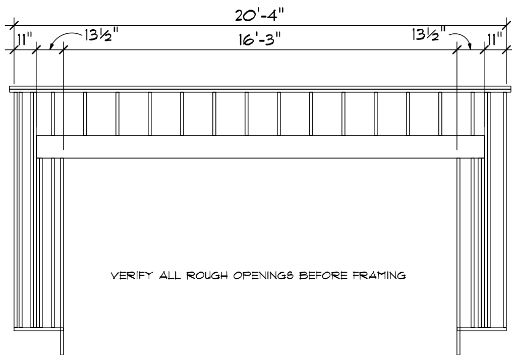
2x4 WALL NO. 1 MAIN
