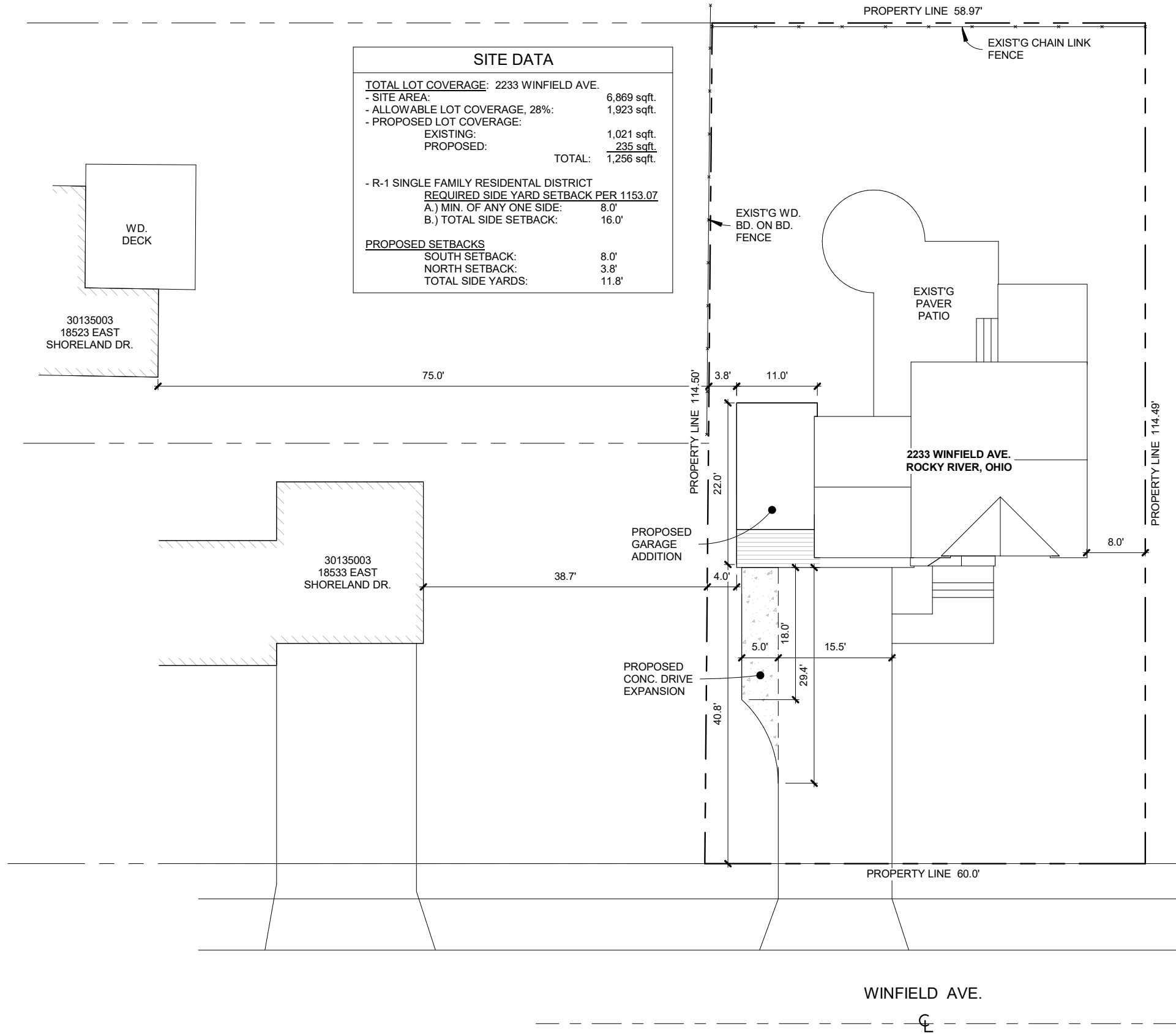
SITE PLAN 1/16" = 1'-0"
