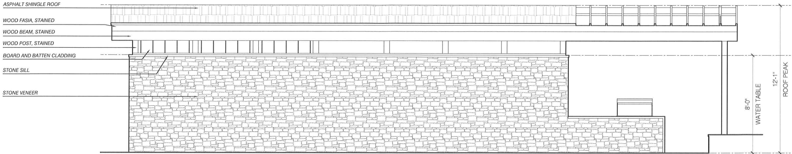
BACK ELEVATION
