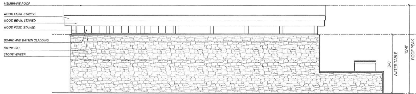
BACK ELEVATION
