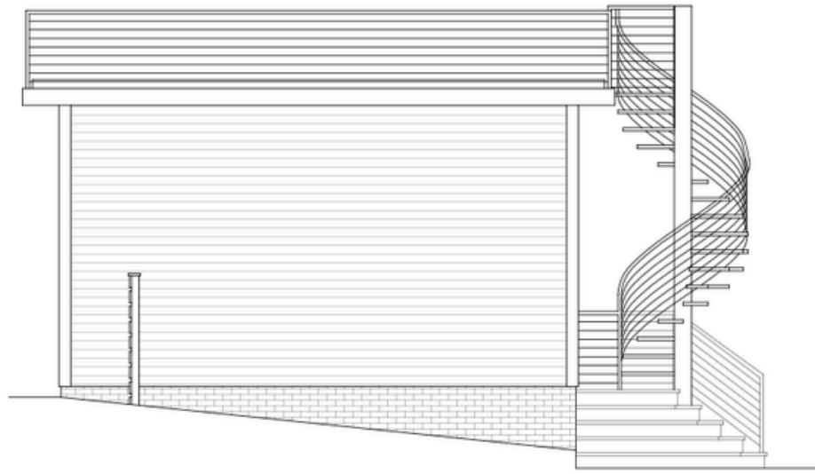
1 PROPOSED EAST ELEVATION 1/4" = 1'-0"
