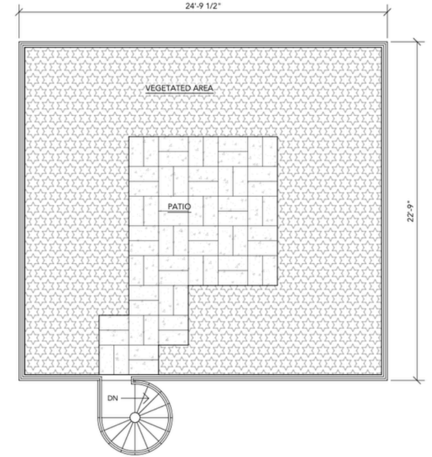
5 PROPOSED ROOF PLAN 1/4" = 1'-0"
