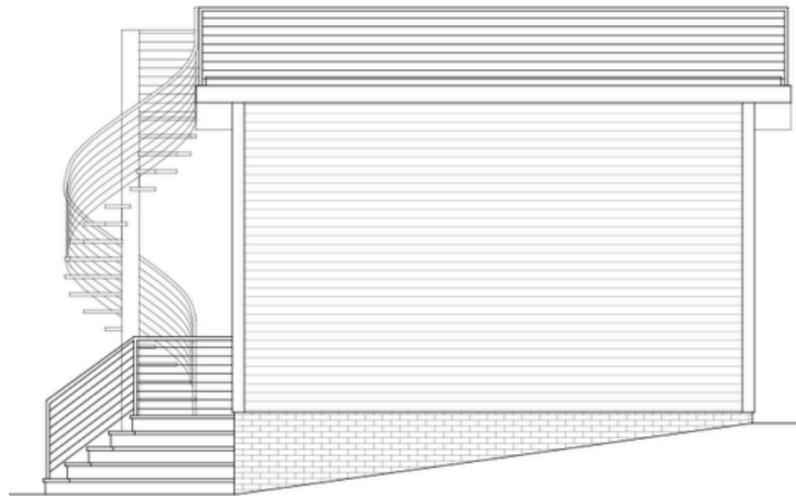
3 PROPOSED WEST ELEVATION 1/4" = 1'-0"
