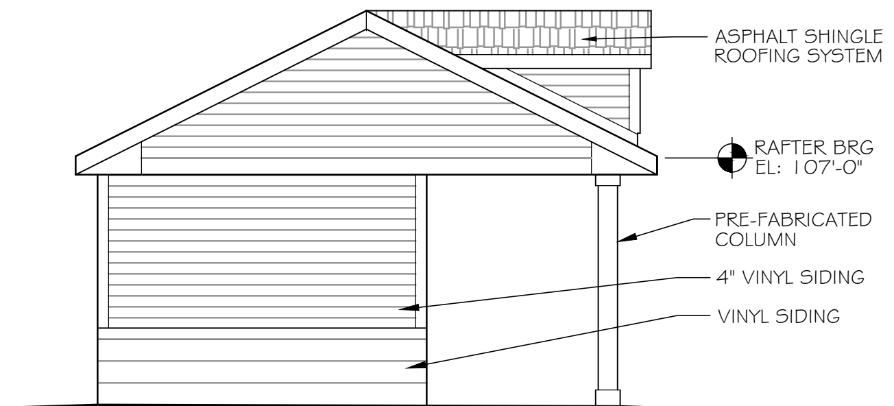
NORTH (side) ELEVATION/ SOUTH SIM.
