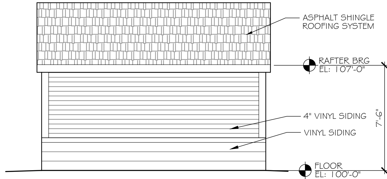
EAST (back) ELEVATION
