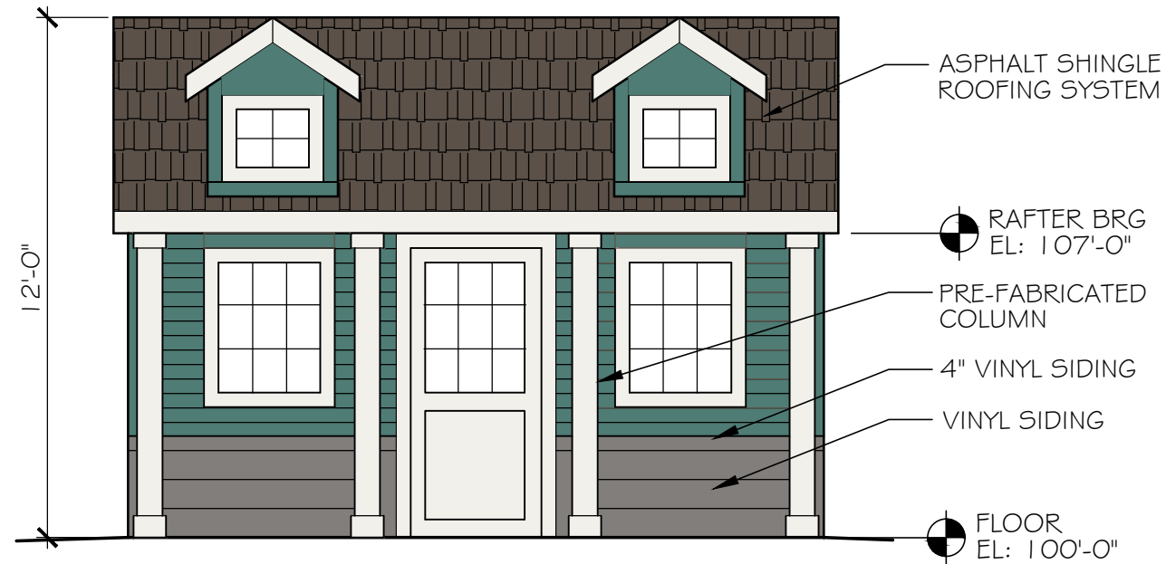
WEST (front) ELEVATION
