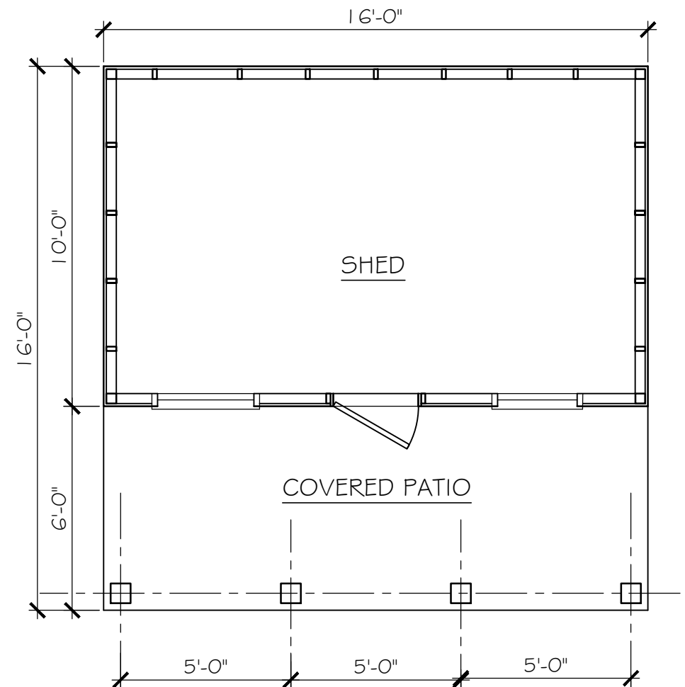
FLOOR PLAN
