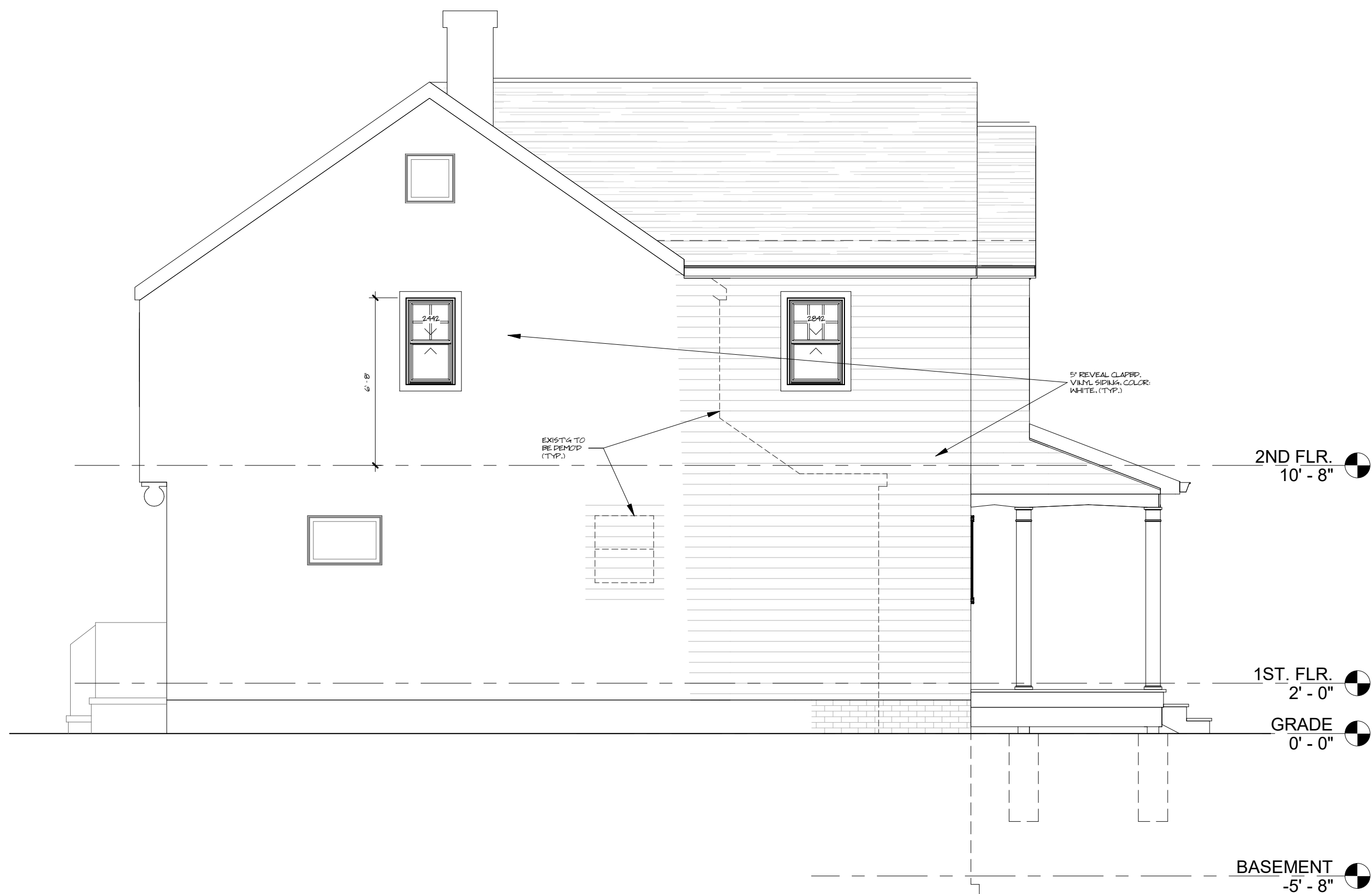
WEST ELEVATION 1/4" = 1'-0"
