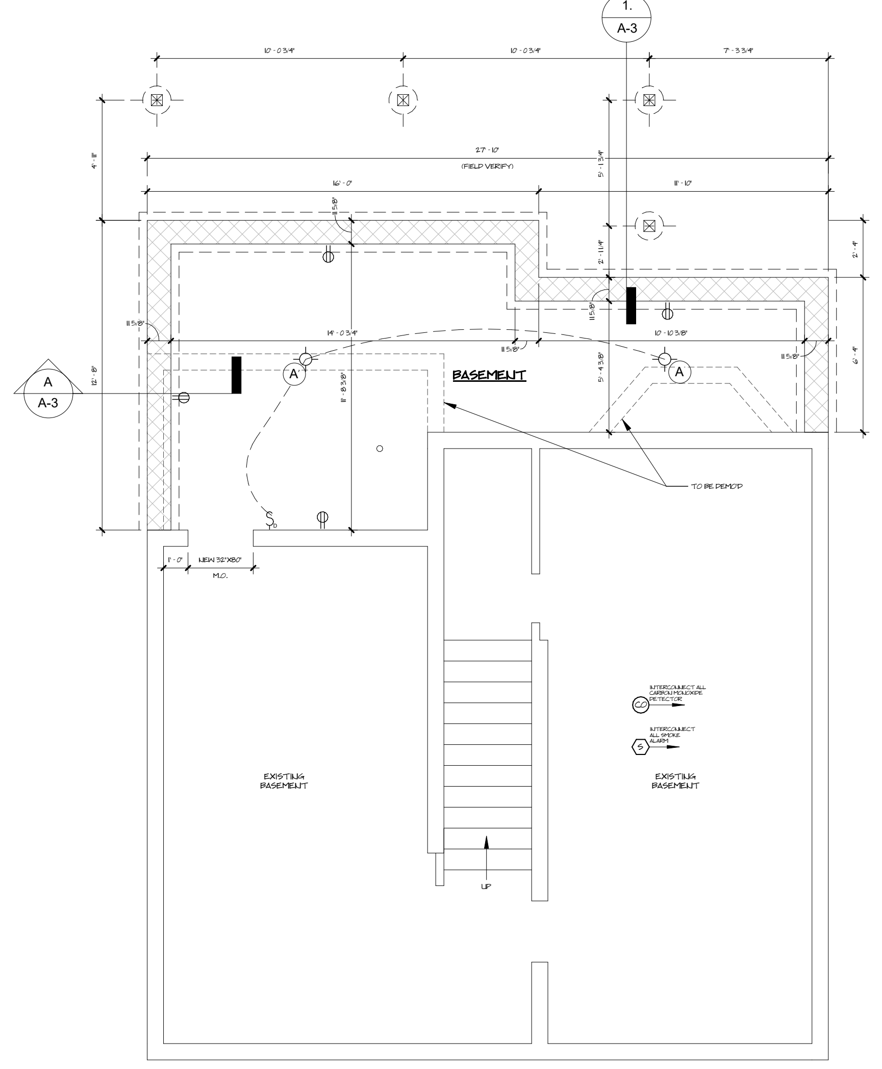
FOUNDATION PLAN 1/4" = 1'-0"
