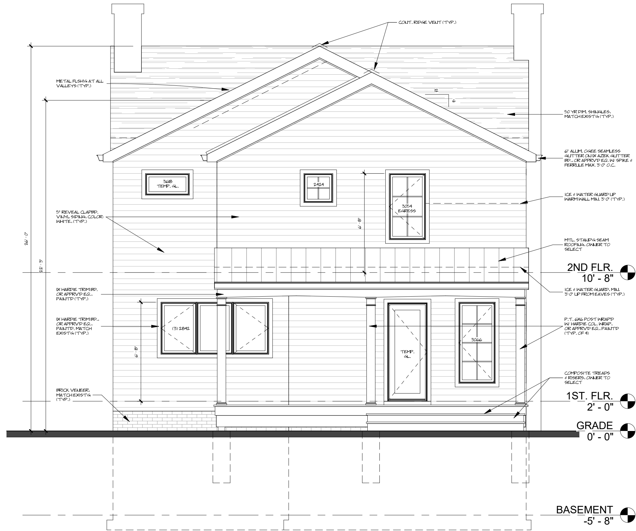
SOUTH ELEVATION 1/4" = 1'-0"
