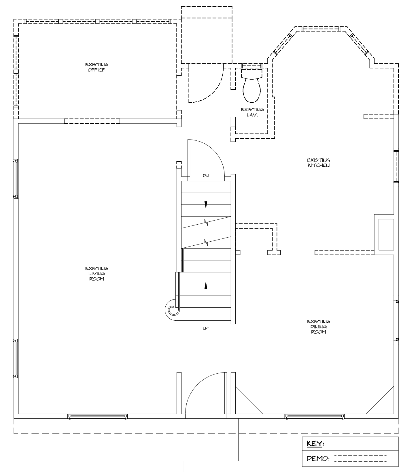
FIRST FLOOR DEMO PLAN 1/4" = 1'-0"
