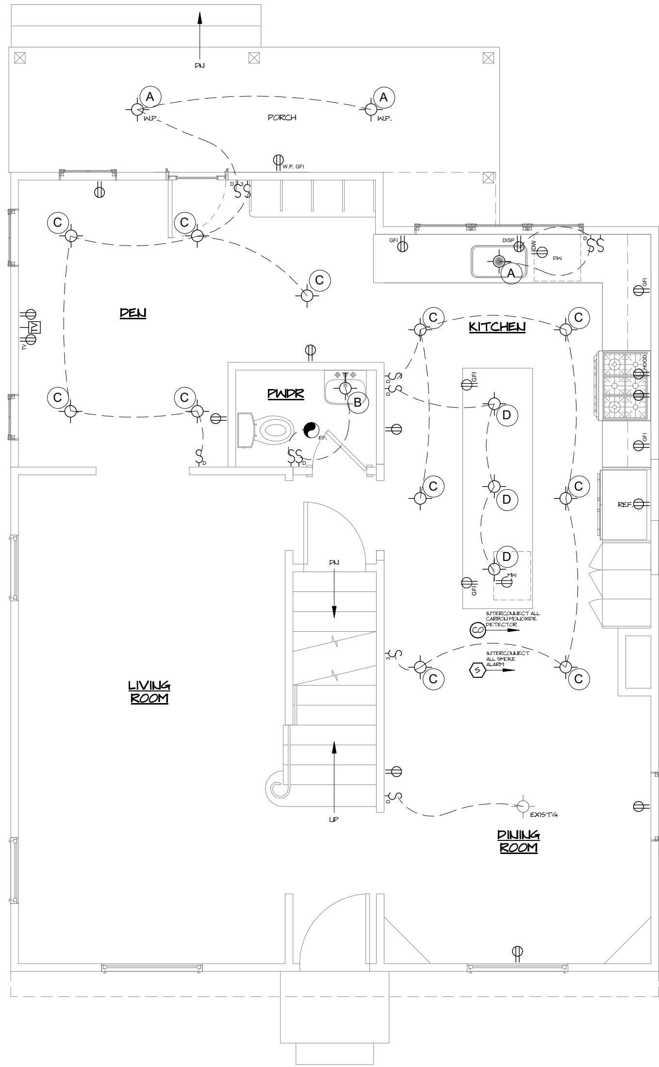
FIRST FLOOR POWER/LIGHTING PLAN 1/4" = 1'-0"
