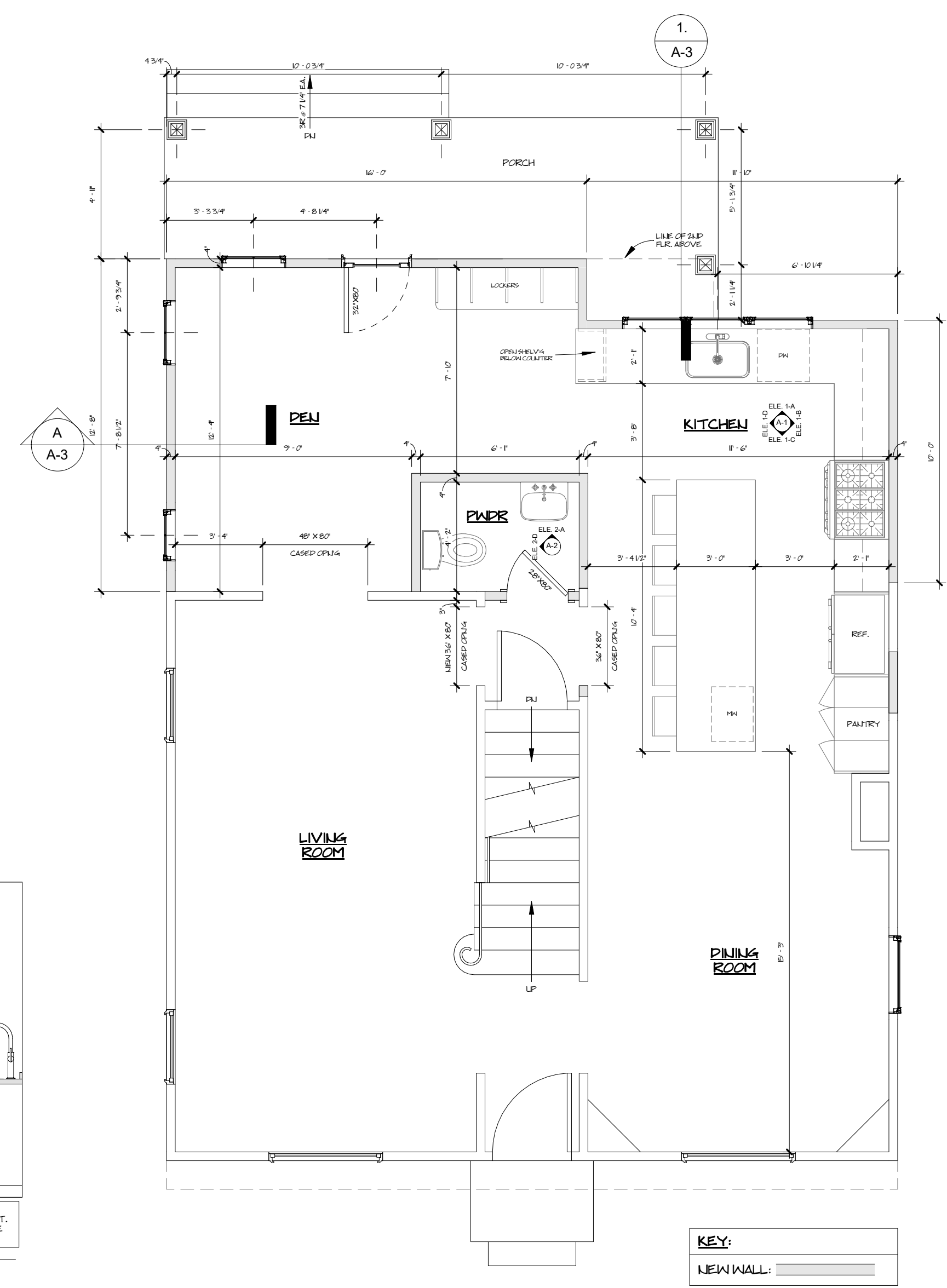
FIRST FLOOR PLAN 1/4" = 1'-0"
