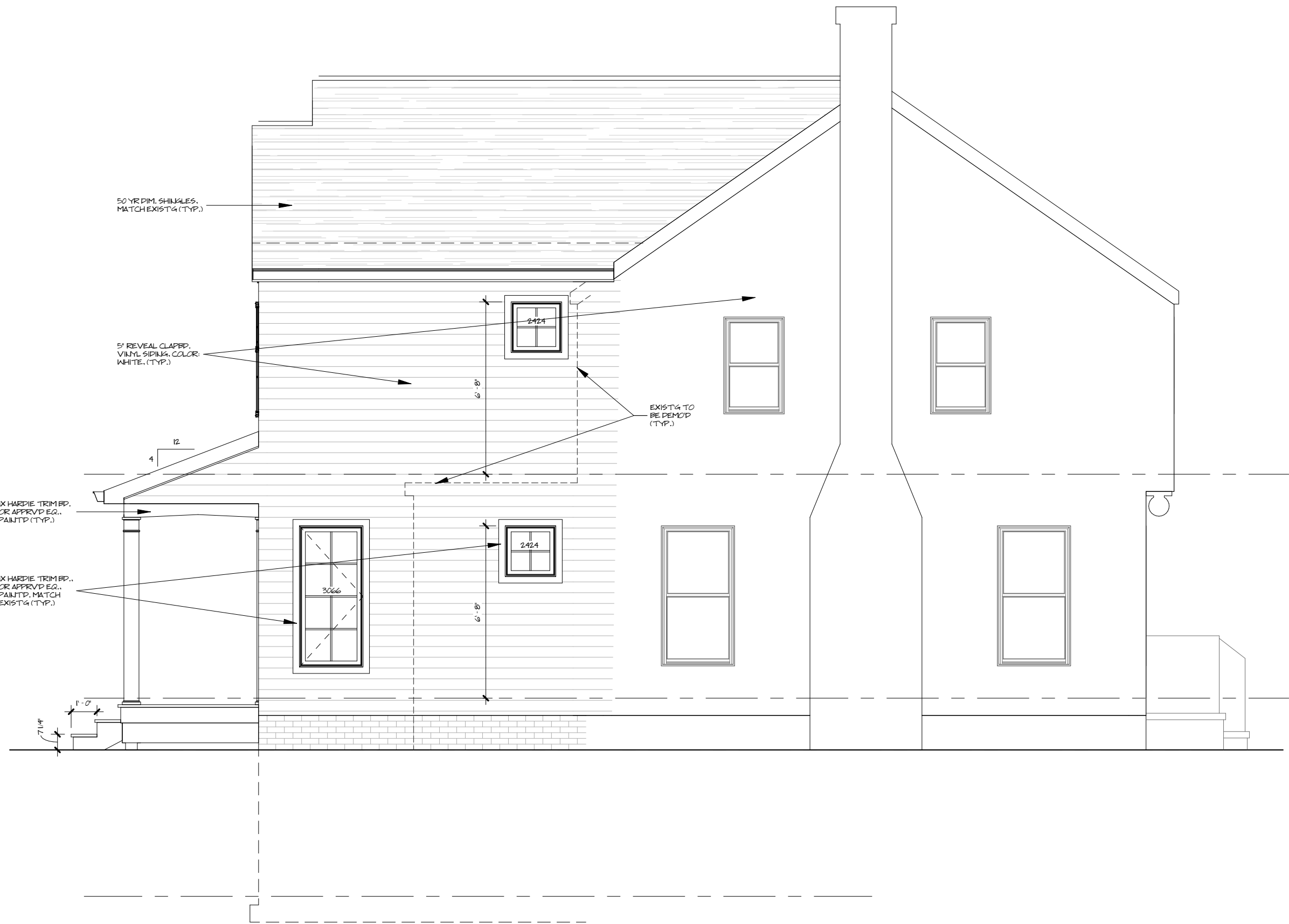
EAST ELEVATION 1/4" = 1'-0"
