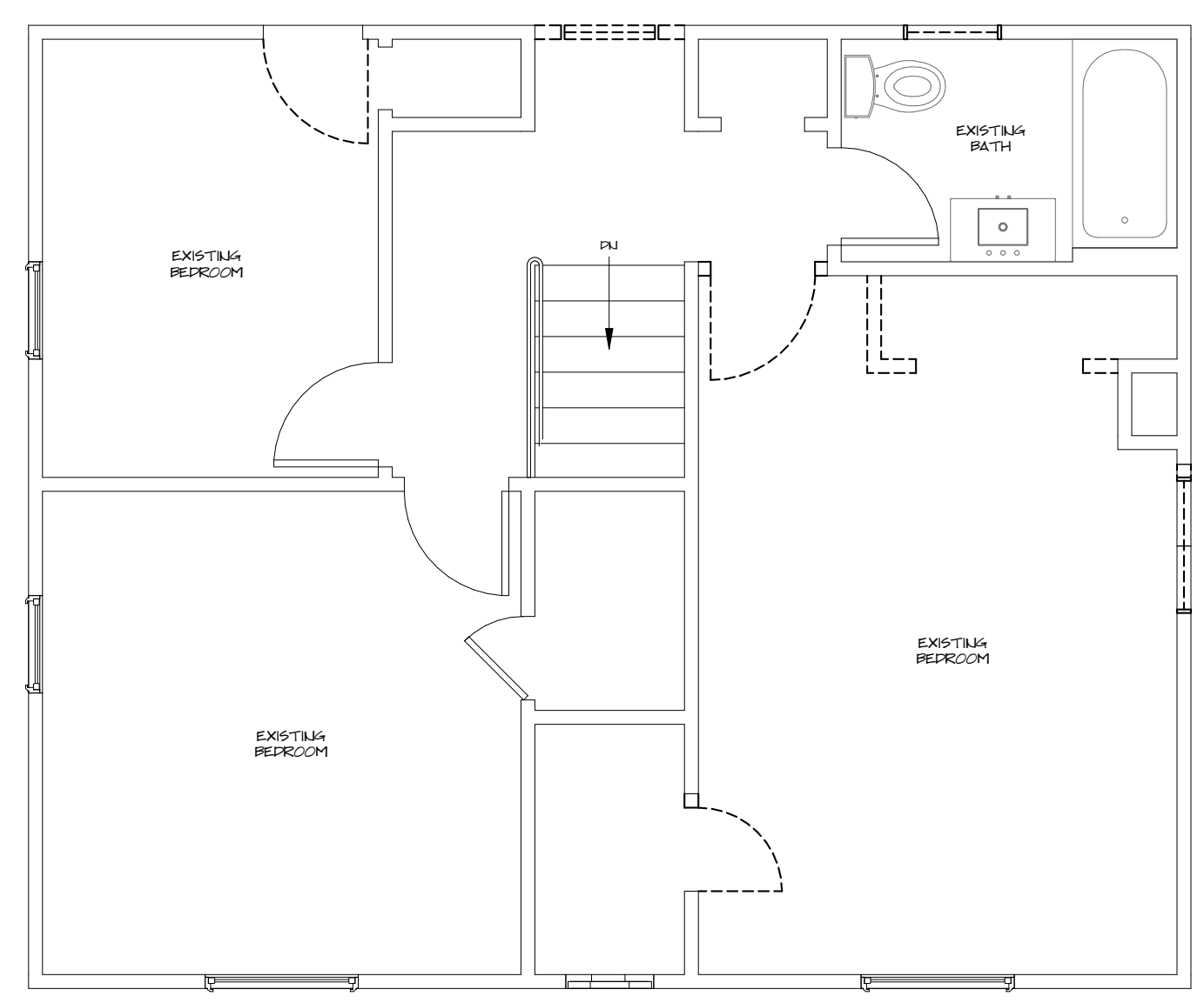
SECOND FLOOR DEMO PLAN 1/4" = 1'-0"
