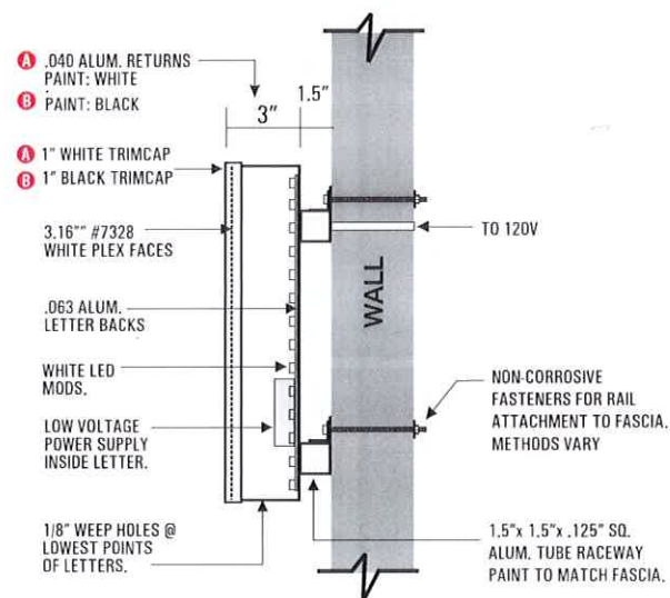
SECTION-THRU "AA" CHANNEL LETTERS ON RAILS
