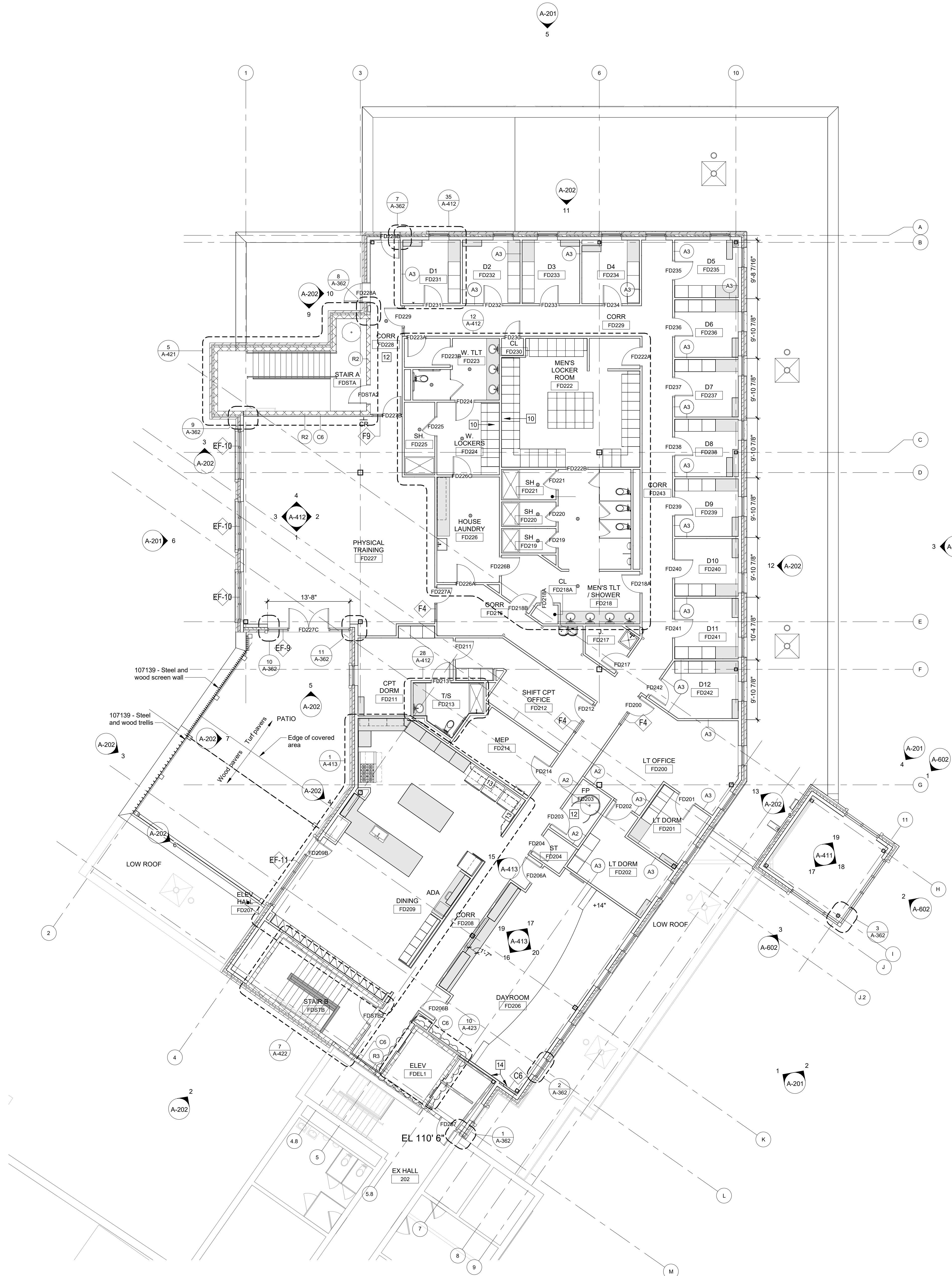
1 FLOOR PLAN - SECOND FLOOR A-112 9, 739 SF + Patio 864 SF
