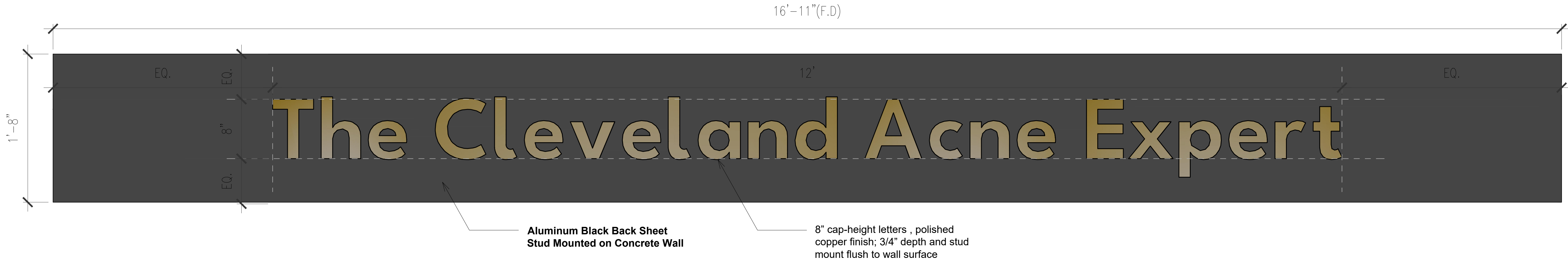
Sign Type XB01 - Building ID Signage - Front View of Signage Scale: 3/4"=1'-0"
