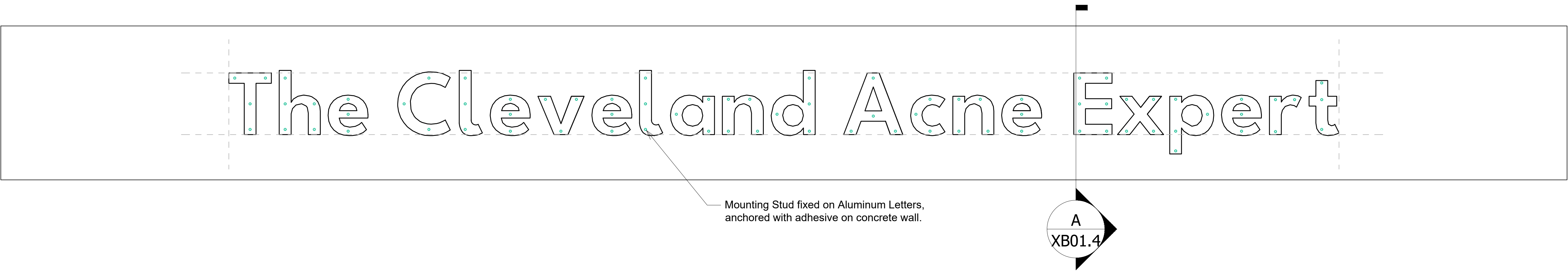
Sign Type XB01 - Building ID Signage - Inside Framing/ Studs Mount Scale: 3/4"=1'-0"
