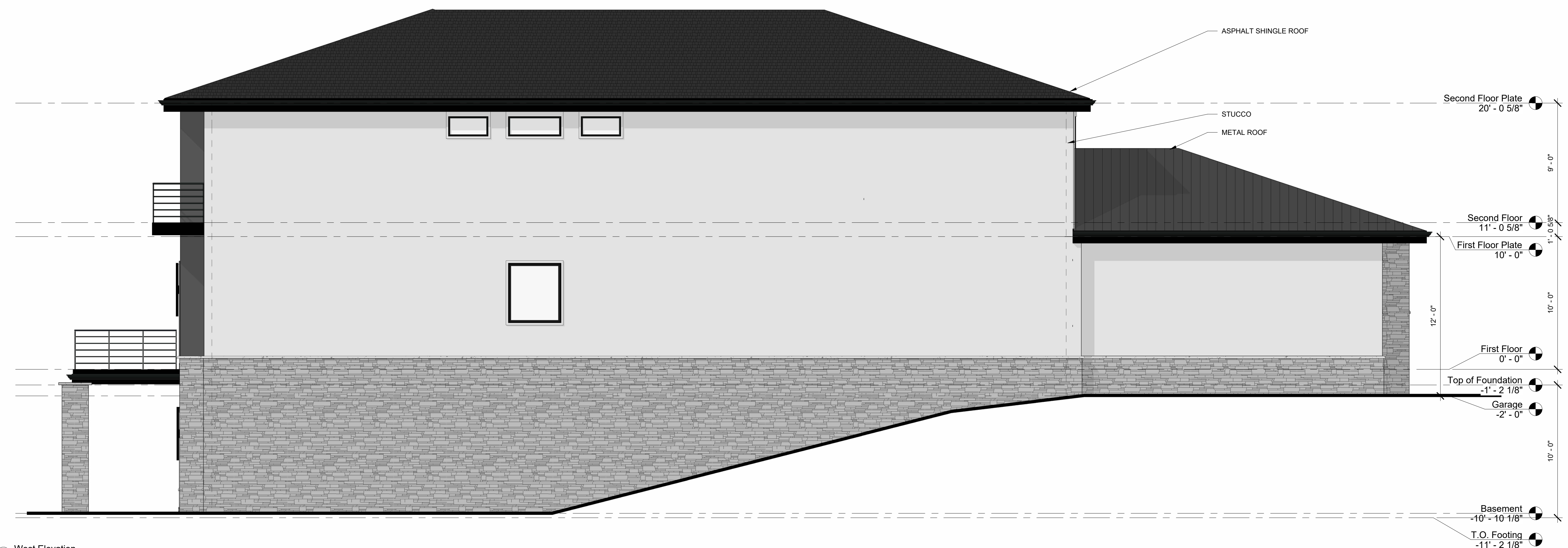
① West Elevation 1/4" = 1'-0"
