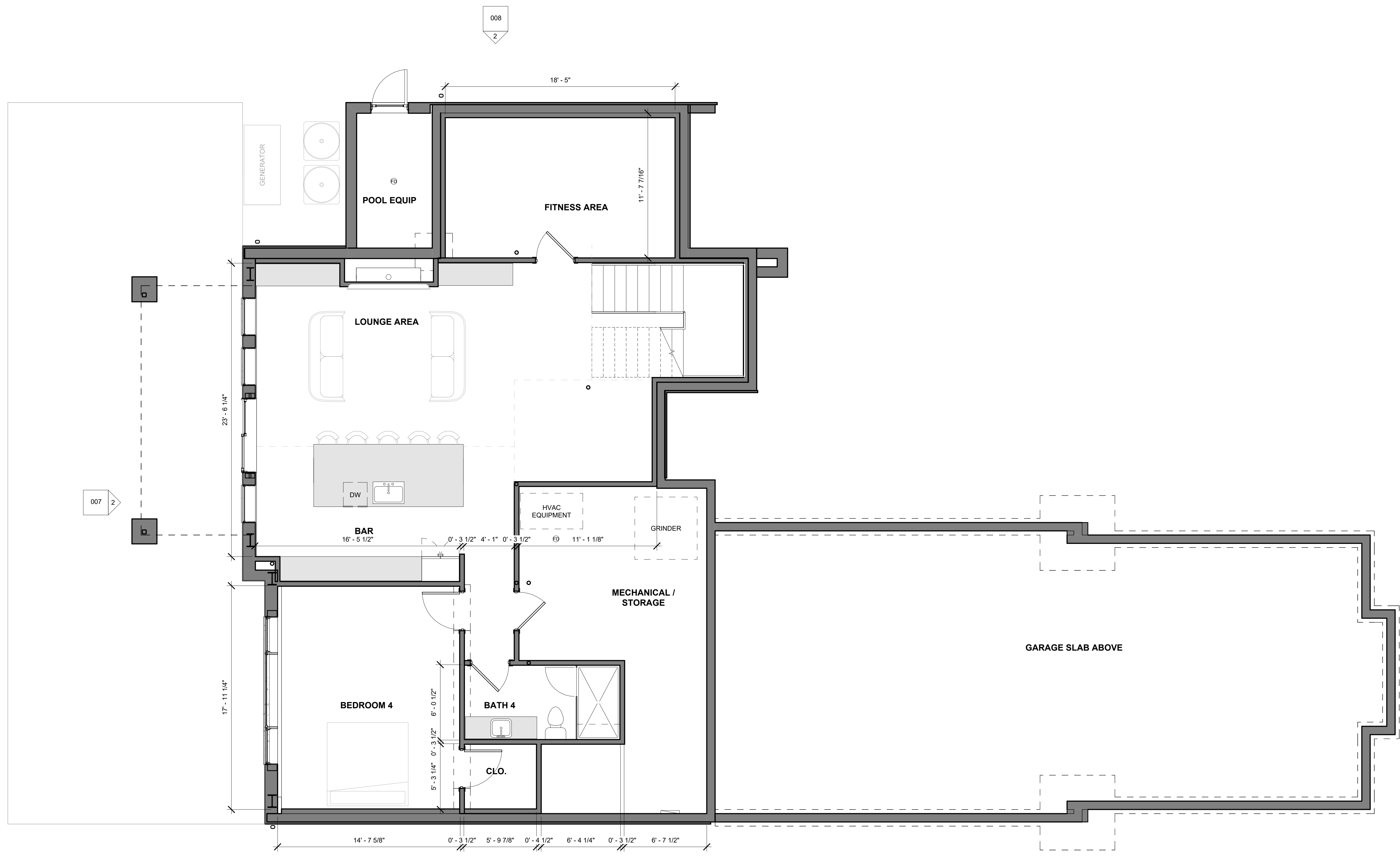
1 Basement Plan 1/4" = 1'-0"
