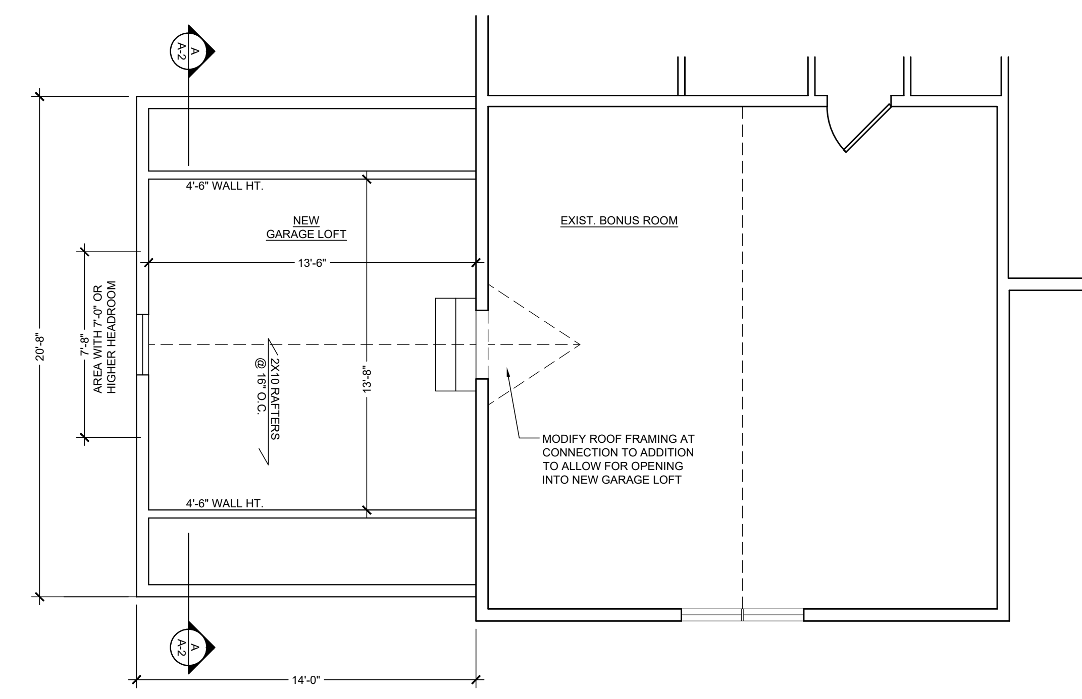
GARAGE LOFT PLAN SCALE: 1/4" = 1'-0"
