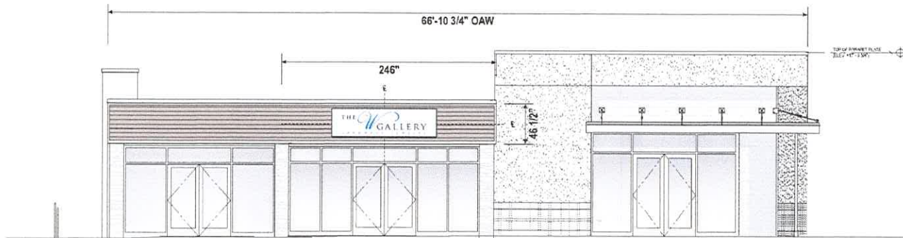
SOUTH ELEVATION 1/8" = 1'-0"
