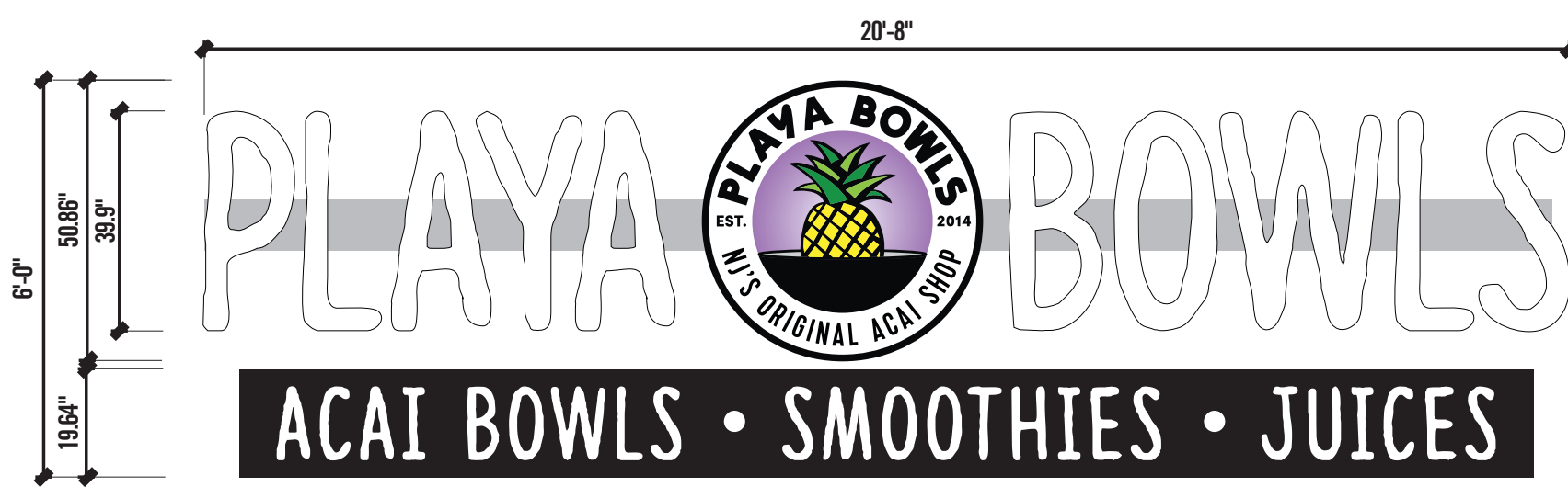
Channel Letters Elevation
