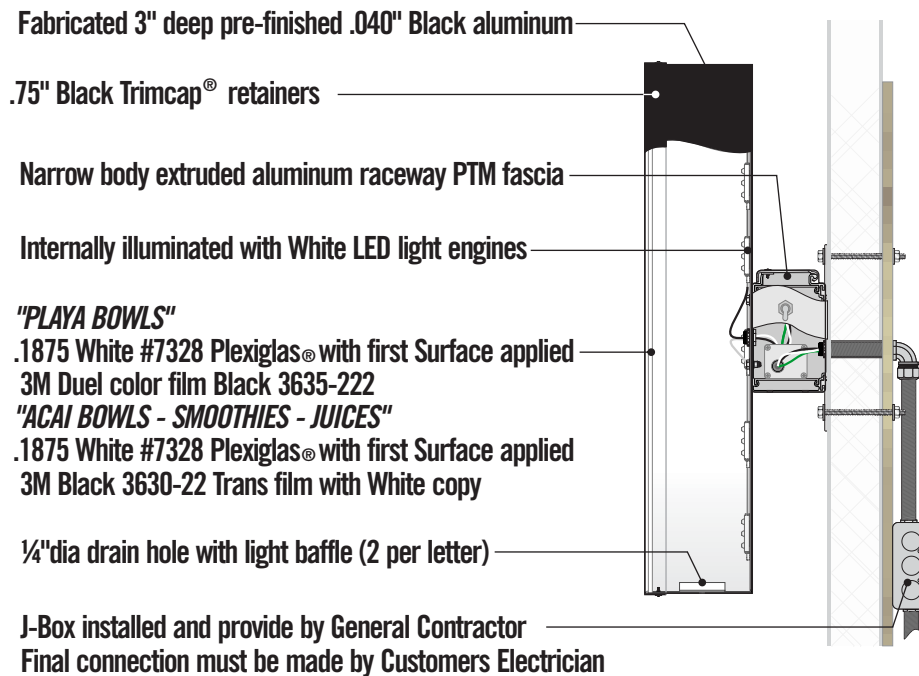
Channel Letter Section
