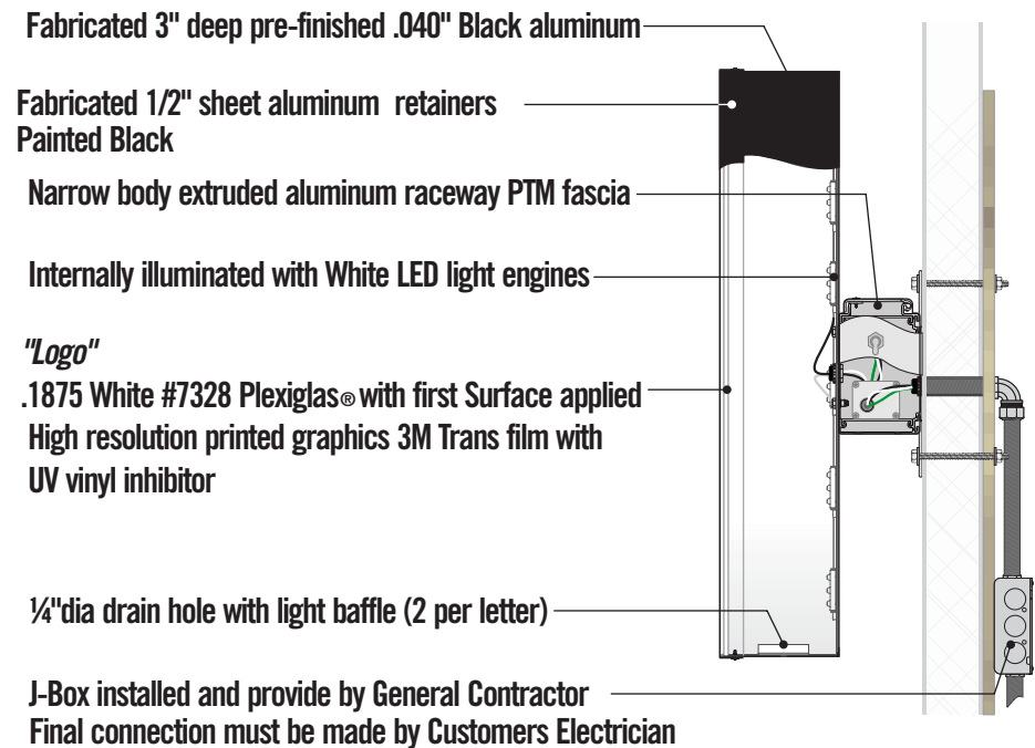
Channel Letter Section - Through Logo
