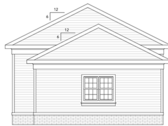
4 PROPOSED SOUTH (SIDE) ELEVATION 1/4" = 1'-0"
