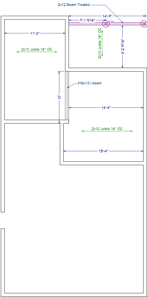
Basement Framing 1st Floor Bearing Detail
