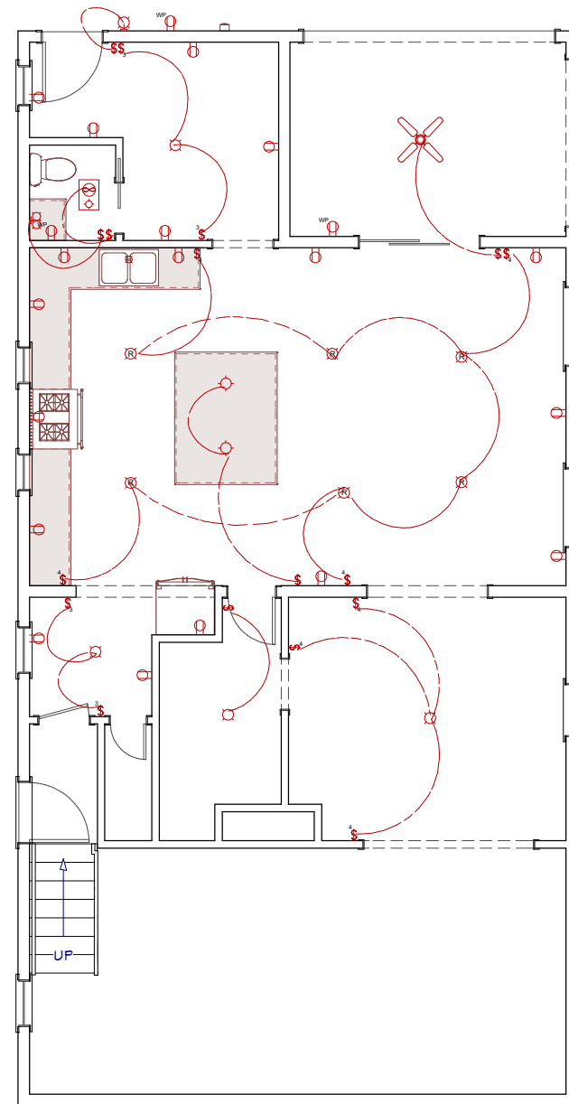
Electrical Plan View
