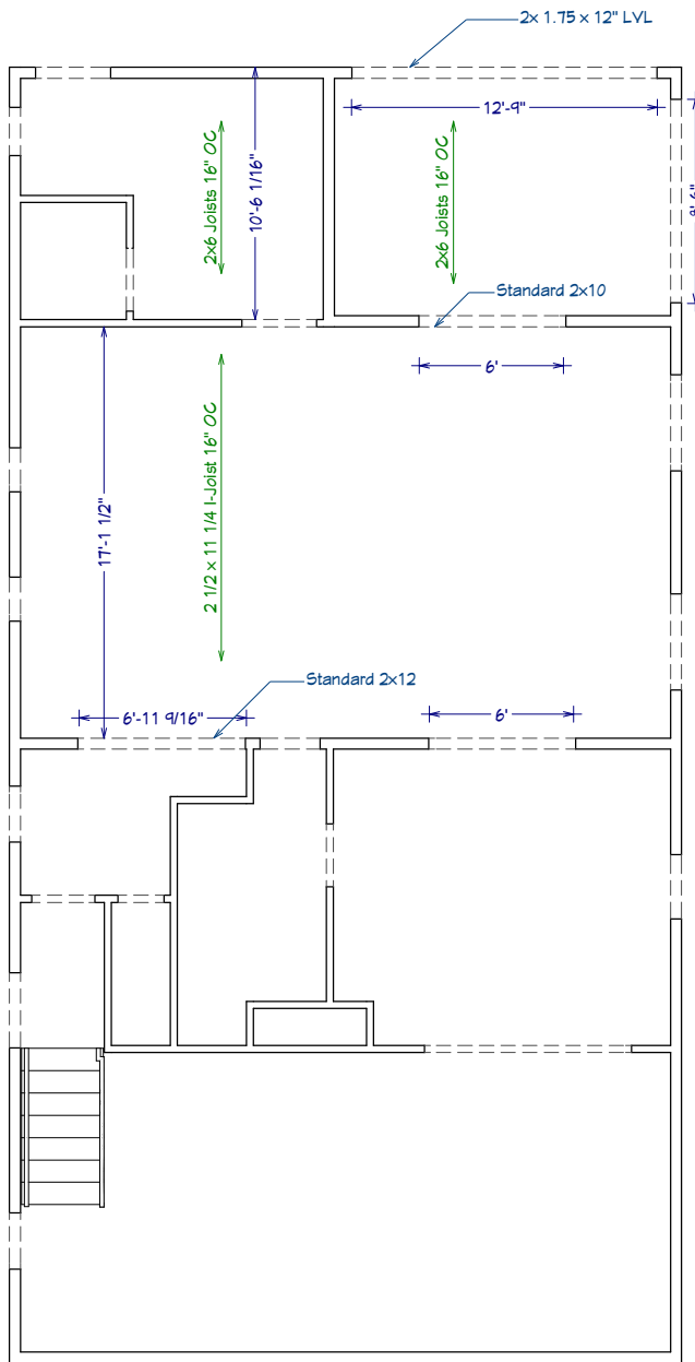
1st Floor Framing/ 2nd Floor Bearing Detail
